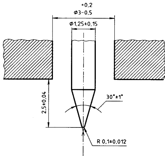
Figure 2 — Indenter for type D durometer
